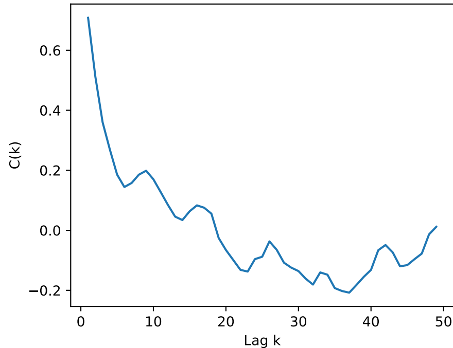
LUMO Autocorrelation
